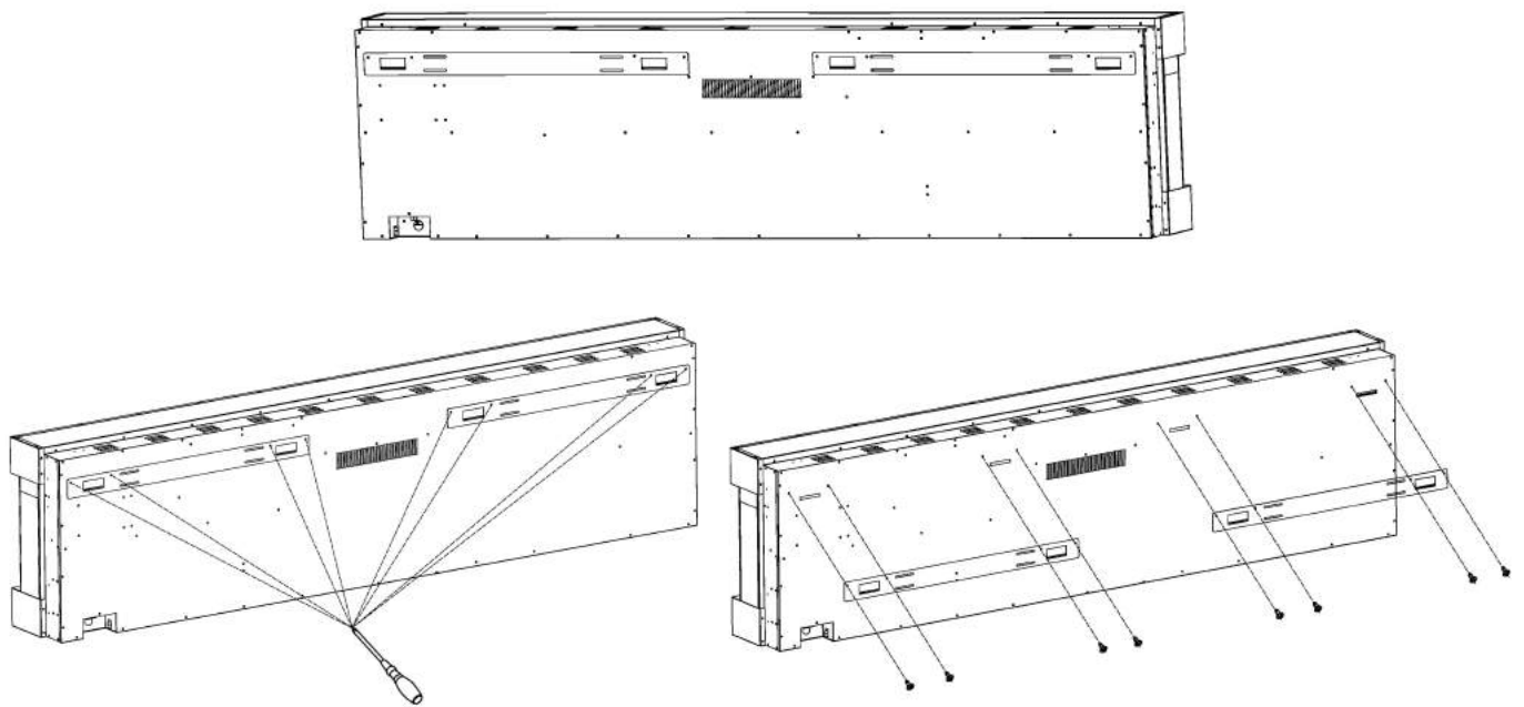
BEF-60-72WMT02 Wall Bracket Illustrated
